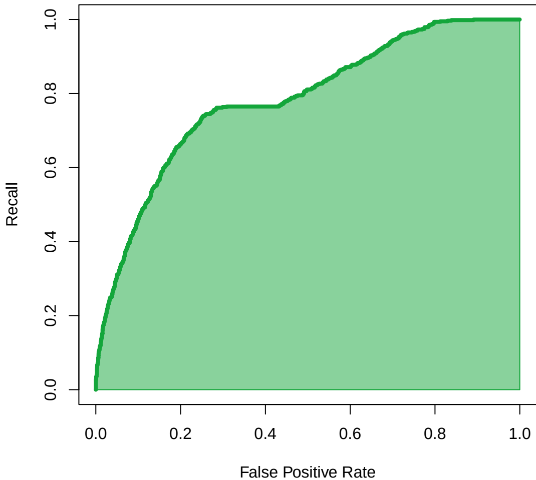
Example ROC Curve
